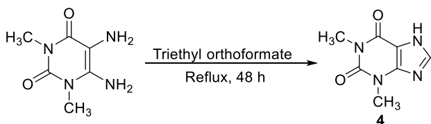
Scheme 4. Synthesis of Theophylline.
