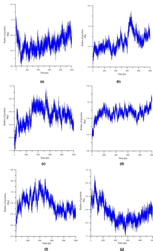
Figure 5. Variations in the Radius of Gyration of Molecules in the Molecular Dynamics Simulation of SCF (a), SCF-(His)6-Myc (b), A2-SCF-(His)6-Myc (c), B-SCF-(His)6-Myc (d), E-SCF-(His)6-Myc (e), M-SCF-(His)6-Myc (f).
