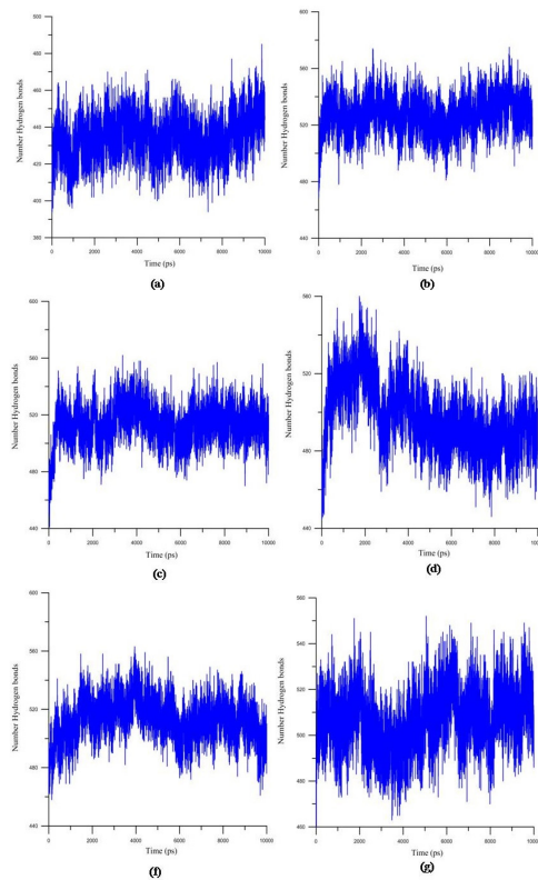
Figure 7. The Number of Hydrogen Bonds Between the Atoms of SCF (a), SCF-(His)6-Myc (b), A2-SCF-(His)6-Myc (c), B-SCF-(His)6-Myc (d), E-SCF-(His)6-Myc (e), M-SCF-(His)6-Myc (f), M-SCF-(His)6-Myc (g).
