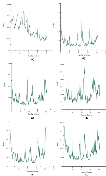
Figure 6. Variations in Root Mean Square Fluctuation of Molecules in the Molecular Dynamics Simulation of SCF (a), SCF-(His)6-Myc (b), A2-SCF-(His)6-Myc (c), B-SCF-(His)6-Myc (d), E-SCF-(His)6-Myc (e), M-SCF-(His)6-Myc (f).
