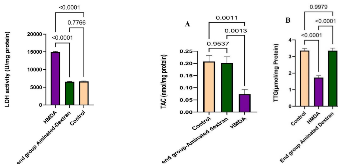
Figure 5. Effect of HMDA and End-Group Aminated Dextran on LDH Activity. Note. HMDA: 1,6-Hexamethylenediamine; LDH: Lactate dehydrogenase; SE: Standard error of the mean; ANOVA: Analysis of variance. The data are displayed as mean \pm SE. P < 0.05 is considered statistically significant. Groups were compared with each other using ANOVA and Tukey's test
