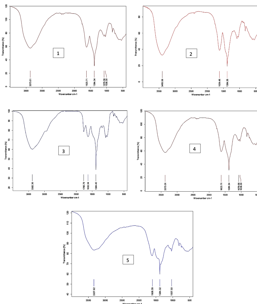
Figure 3. The IR Spectra of the 5 Complexes.
