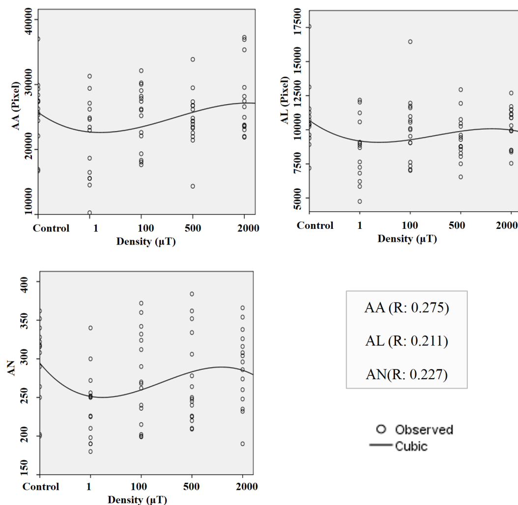
Figure 2. Correlation of AA, AL and, AN with an increase in the magnetic flux densities of 50-Hz MFs. Note. MF: Magnetic fields. A curve estimation analysis was performed to evaluate the correlation of AA, AL, and AN with the increase of the magnetic flux densities from 1 to 100, 500, and 2000 \mu\text{T} . There were regression correlations (cubic model) among AA, AL, and AN with the magnetic flux densities.
