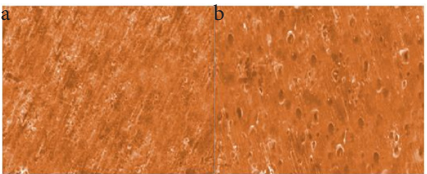
Figure 5. Scanning Electron Photomicrographs of Tablet (a) Obtained Before Dissolution and (b) Porous Region of Membrane Containing 10% w/w PEG-400. Note. PEG-400: Polyethylene glycol 400.
