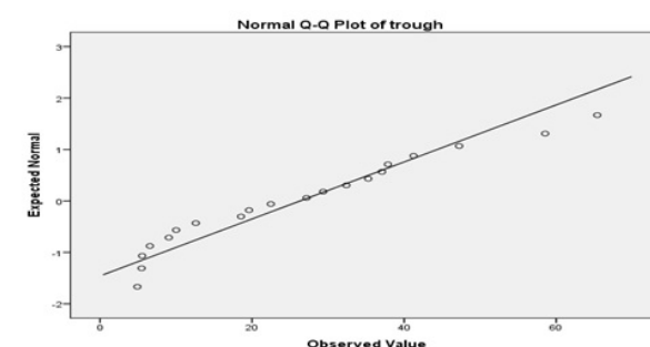
Figure 4. Normal Q-Q Plot of Trough Data. Note. Q-Q: Quantile-quantile.
