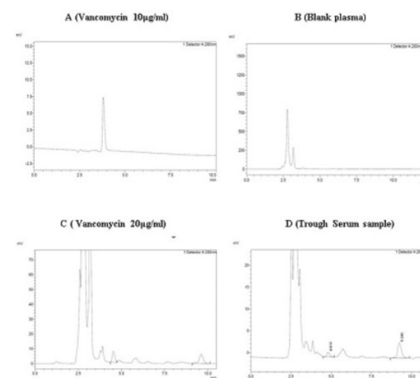
Figure 3 . (A) HPLC Chromatograms of Vancomycin 10 \mu\text{g/mL} , (B) Blank Plasma, (C) Vancomycin and Caffeine 20 \mu\text{g/mL} Spiked in Plasma, and (D) Human Trough Sample (5.54 \mu\text{g/mL} ). Note. HPLC: High-performance liquid chromatography.
