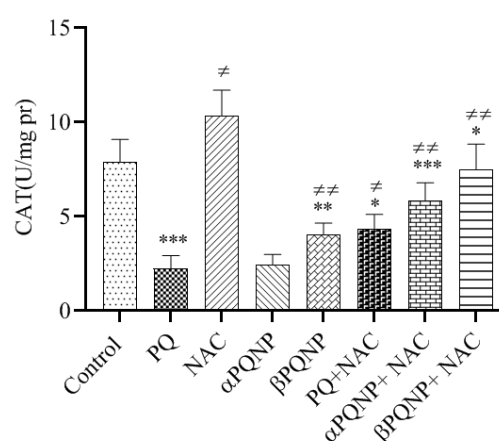
Figure 3: Effects of Nanoparaquat on the Catalase (CAT) Concentration in Brain Homogenate.
