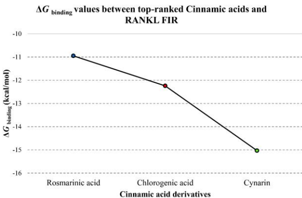
Figure 2. Comparison of calculated \Delta G_{\text{binding}} energies (kcal/mol) for Cynarin (Green), Chlorogenic Acid (Red), and Rosmarinic Acid (Blue) Bound to the RANKL FIR. Abbreviations: RANKL, receptor activator of nuclear factor- \kappa B ligand; FIR, functional inhibitory residues.
