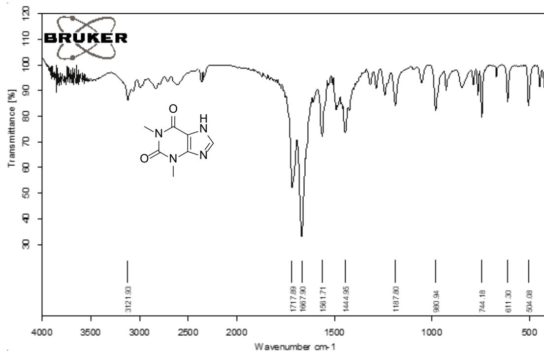
Figure S10: FT-IR spectrum of the theophylline.
