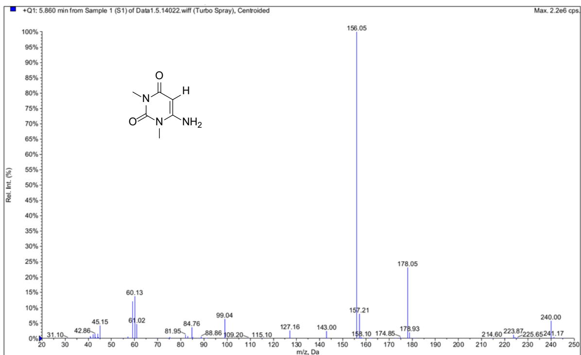
Figure S3: Mass spectrum of the 6-amino-1,3-dimethylpyrimidine-2,4-dione.
