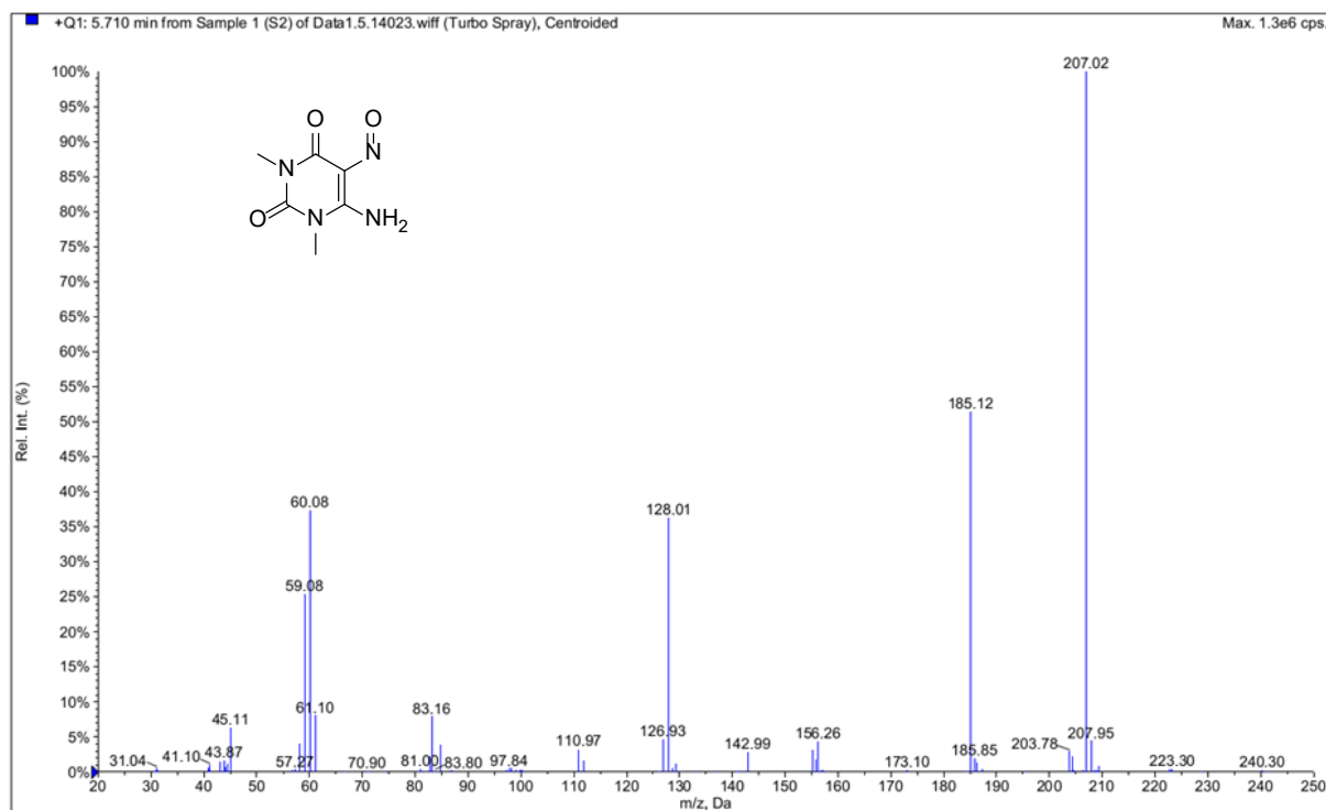
Figure S6: MASS spectrum of the 6-Amino-1,3-dimethyl-5-nitroso-uracil.
