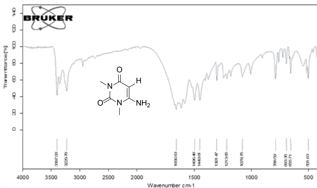
Figure S1: FT-IR spectrum of the 6-amino-1,3-dimethylpyrimidine-2,4-dione.
