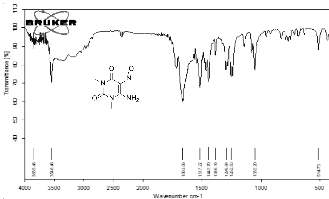
Figure S4: FT-IR spectrum of the 6-Amino-1,3-dimethyl-5-nitroso-uracil.
