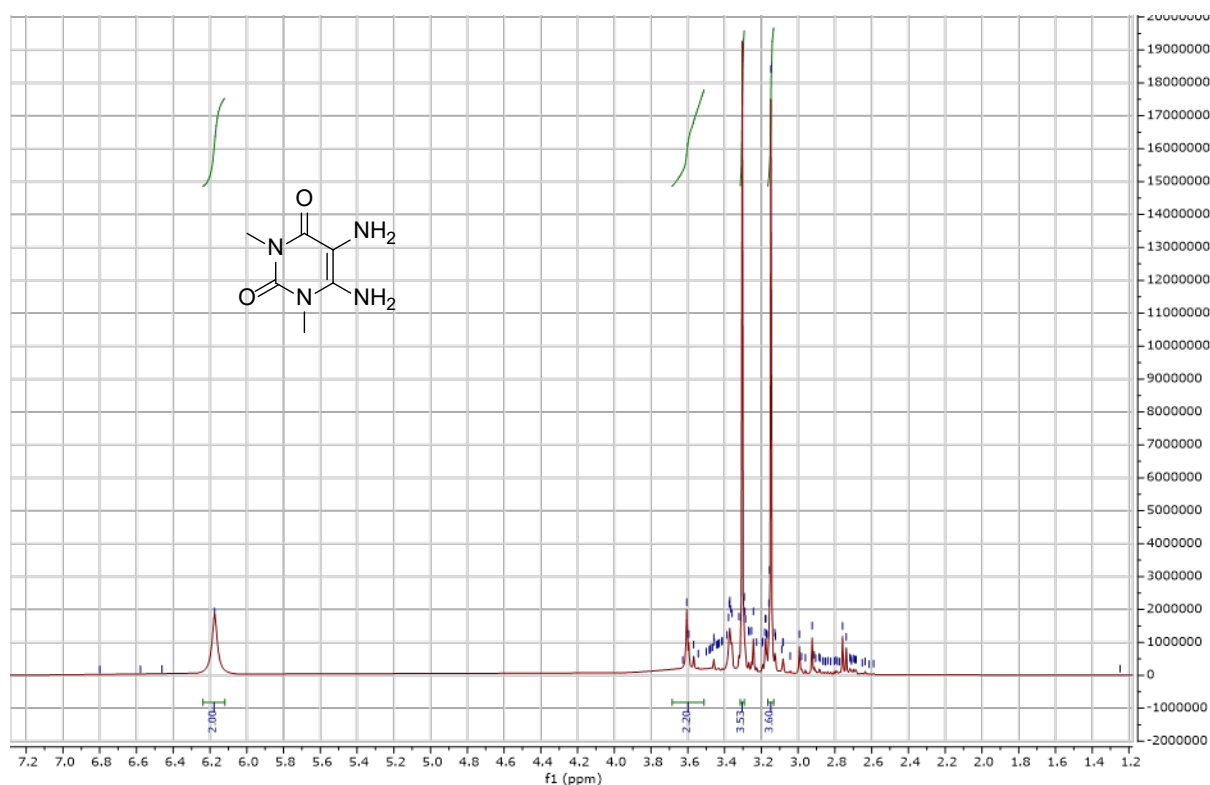
Figure S8: 1 H-NMR spectrum of the 5,6-diamino-1,3-dimethyl uracil.
