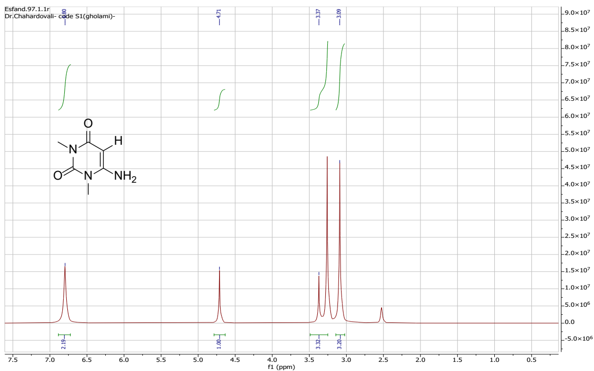
Figure S2: ^1\text{H} -NMR spectrum of the 6-amino-1,3-dimethylpyrimidine-2,4-dione.
