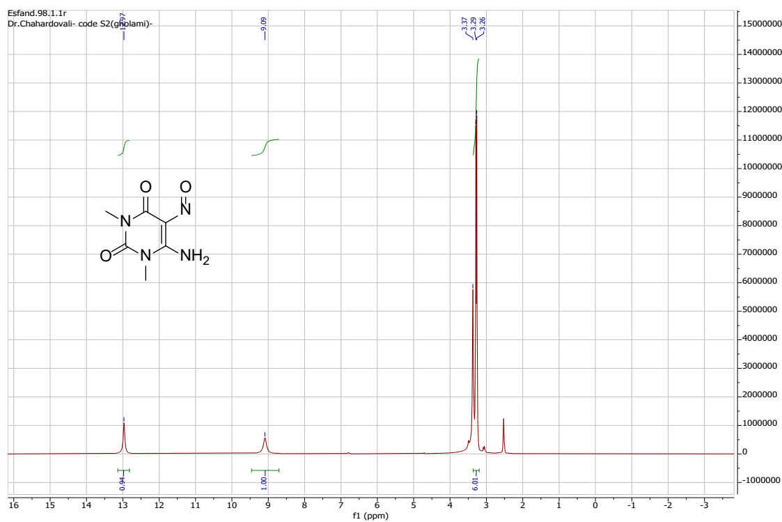
Figure S5: 1 H-NMR spectrum of the 6-Amino-1,3-dimethyl-5-nitroso-uracil.
