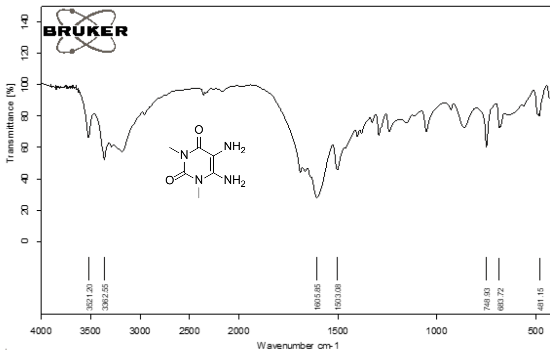
Figure S7: FT-IR spectrum of the 5,6-diamino-1,3-dimethyl uracil.
