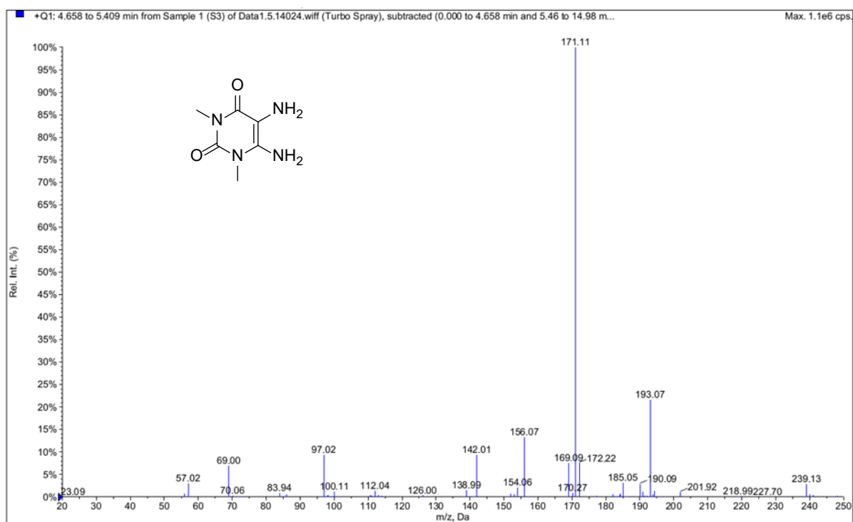
Figure S9: Mass spectrum of the 5,6-diamino-1,3-dimethyl uracil.
